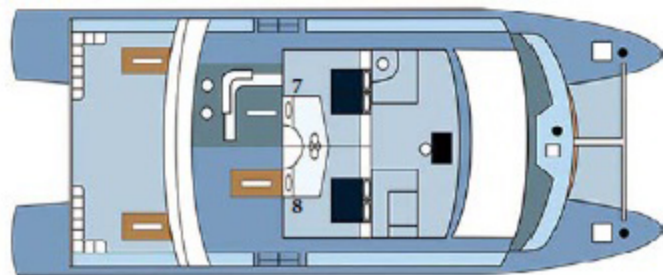
UPPER DECK
